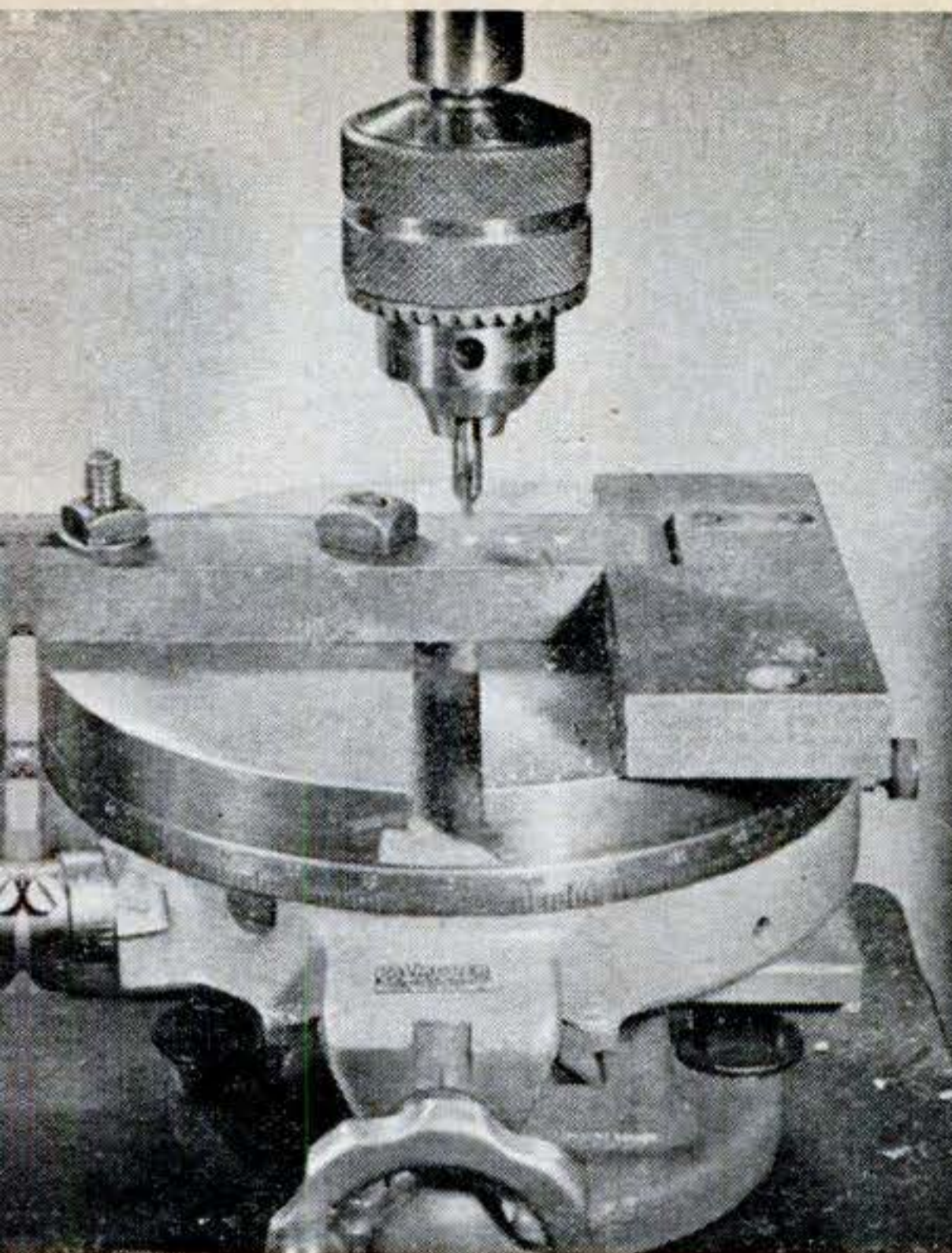
CALIBRATED FEED SCREWS make it possible to position holes to close tolerances. Start the holes with a center-drill, follow with twist drill.
